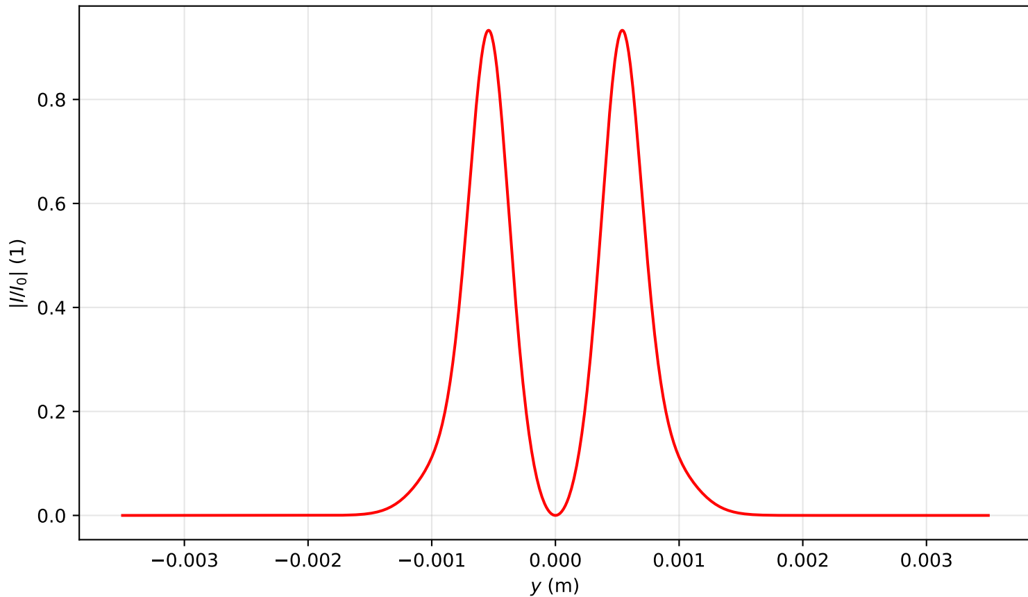
Intensity profile I(x=0, y, z=0.637)/I_0 , \text{Pin}=4.0\text{Pcr} , artificial time
